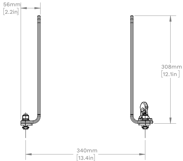
SHOXSTRAXS Lateral Spacing: 340mm [13.4"]
